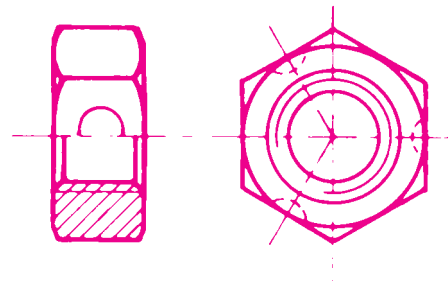
Ecrou hexagonal auto-freiné (DIN 980)
